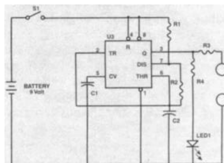
Zapper schematic
